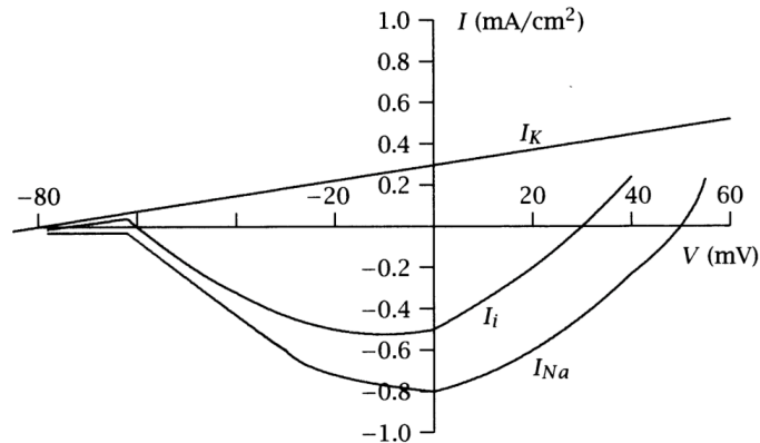
Figure 2: I-V Curve in Squid Axon
