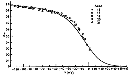
Figure 3: Abscissa: resting potential minus membrane potential. Ordinate: n_\infty calculated from experimental measurements of the steady state potassium conductance I_{K\infty} in the squid giant axon in sea water.
