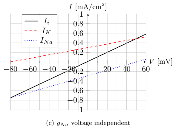
Figure 1: Exercise 5.3: I-V Curve
